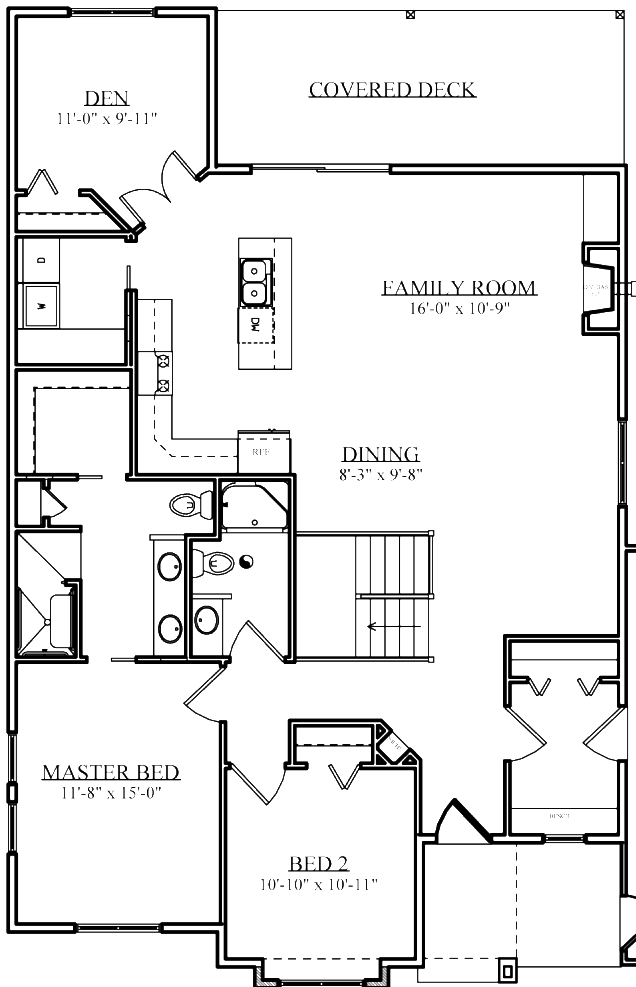
MAIN LEVEL FLOOR PLAN
