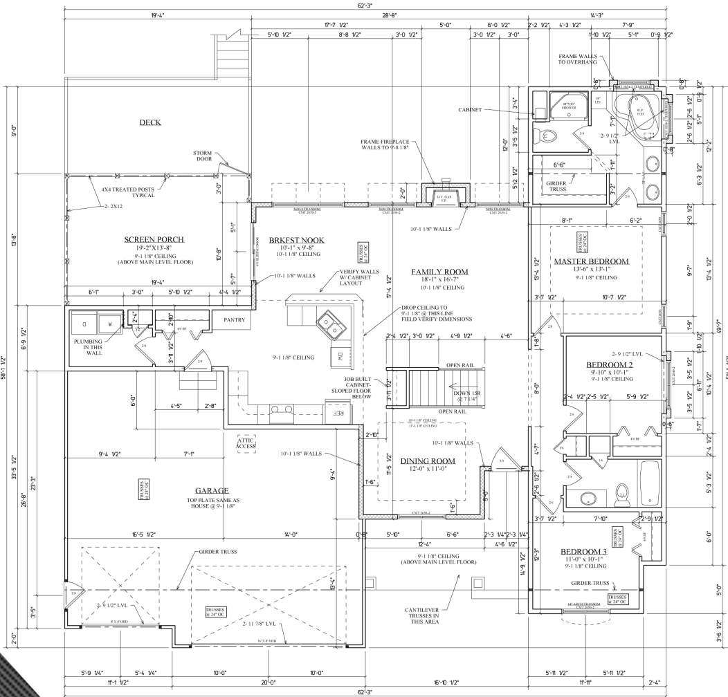
MAIN LEVEL FLOOR PLAN 1,727 SQ. FT.
